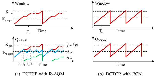
Figure 3. Window Size and Queue Size Process.
