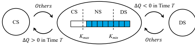
Figure 5. R-AQM state transition diagram
