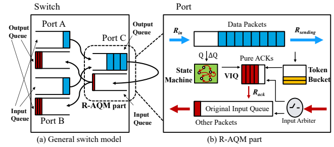
Figure 4. R-AQM design.
