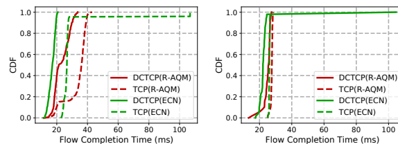
(a) 10-to-1 incast (b) 100-to-1 incast
