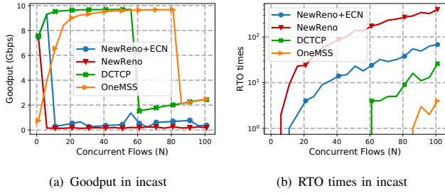
Figure 2. The experiment to show the incast problem.
