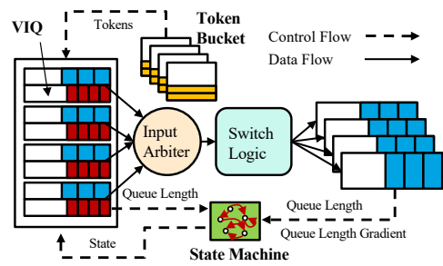
Figure 6. R-AQM switch architecture on NetFPGA-SUME
