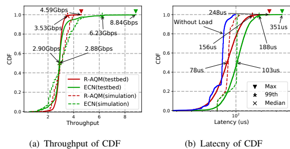
Figure 11. Latency and Throughput of CDF in the incast scenario.
