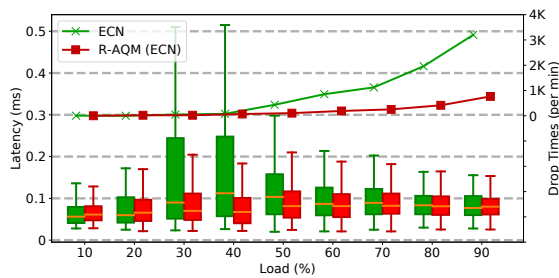
Figure 12. Latency and Drop Times in the all to all scenario (testbed). and provides better fairness.
