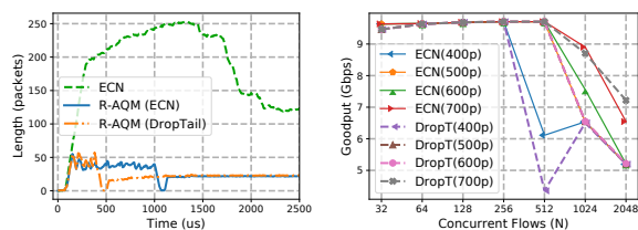
(a) Reaction Details Analysis of R-AQM (b) Sensitivity Analysis of R-AQM
