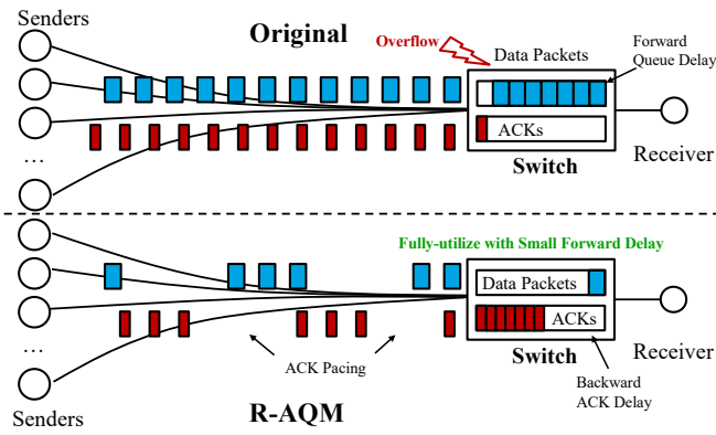
Figure 1. The general idea of R-AQM an illustrative example.
