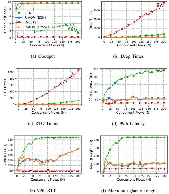
Figure 7. Goodput, Drop times, RTO times, Latency, RTT and Queue Length with many concurrent flows
